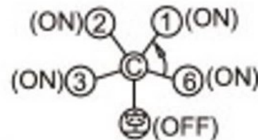
SCHEMATIC (NON-SHORTING)
